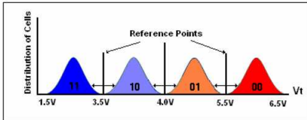
Figure 4: Voltage Reference for MLC
