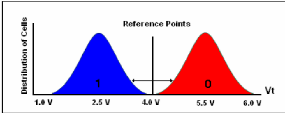
Figure 3: Voltage Reference for SLC
