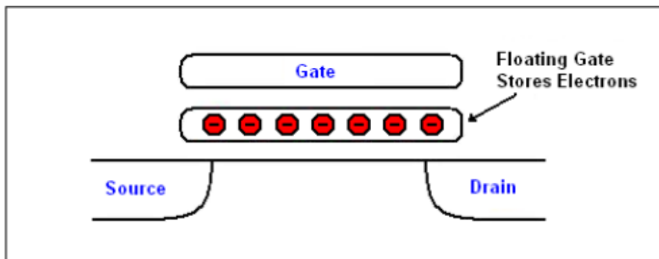
Figure 2: Flash Transistor Cell
